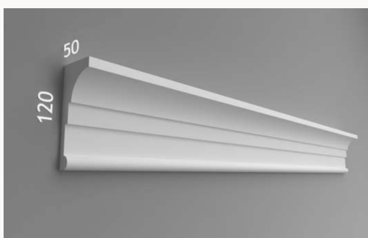
Architrave: WP17
