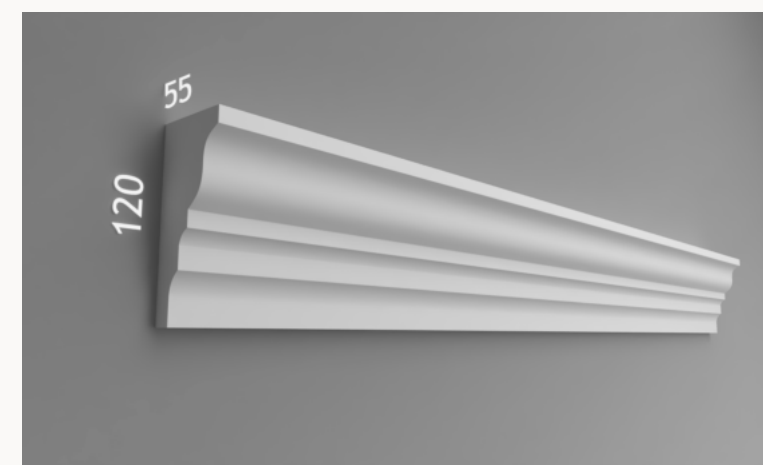
Architrave: WP18
